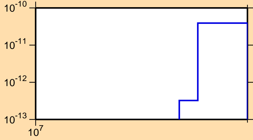
\sigma vs. E for ^{159}\text{Er} (mt 34)
