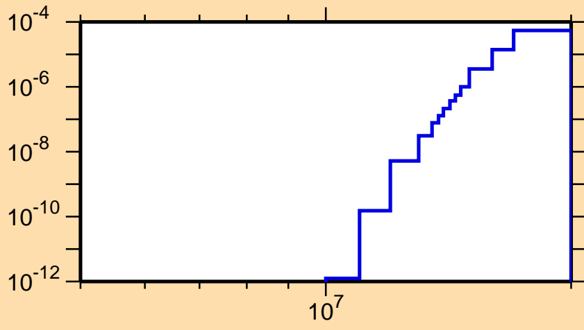
\sigma vs. E for ^{159}\text{Er}(n,2n\alpha)
