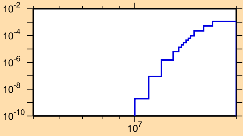
\sigma vs. E for ^{159}\text{Er}(n,t)
