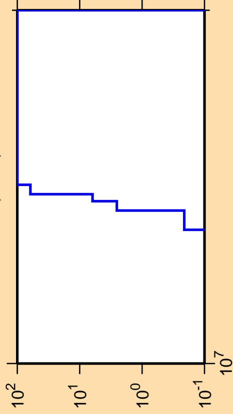
\Delta\sigma/\sigma vs. E for ^{159}\text{Er}(n,nd)
