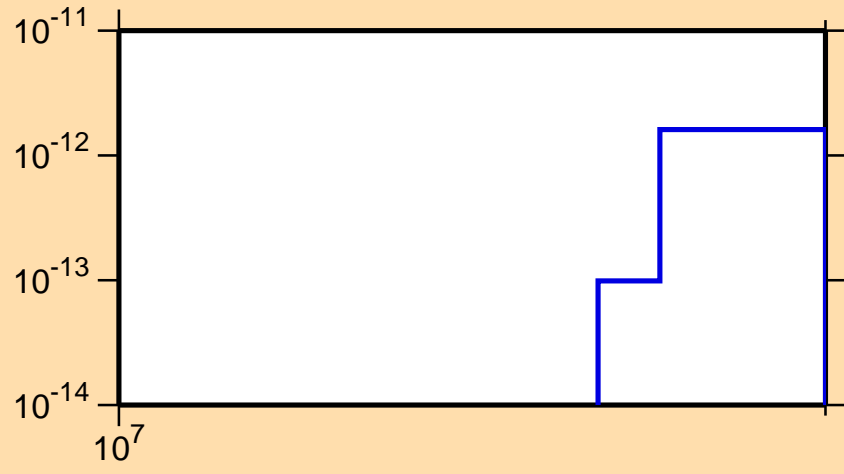
\sigma vs. E for ^{159}\text{Er}(\text{mt117})
