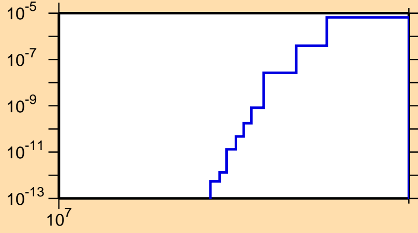
\sigma vs. E for ^{159}\text{Er}(n,nd)
