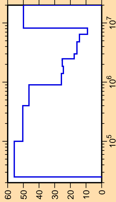
\Delta\sigma/\sigma vs. E for ^{159}\text{Er}(n,\text{inel.})
