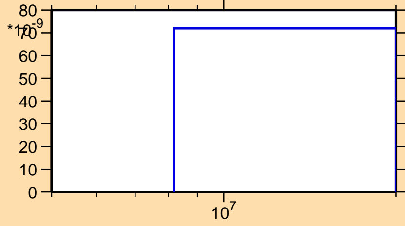
\sigma vs. E for ^{159}\text{Er}(n,\text{nd})
