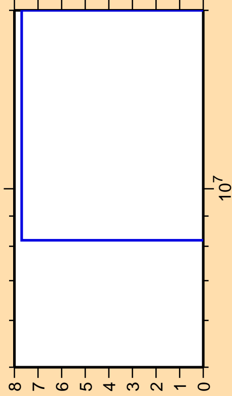
\Delta\sigma/\sigma vs. E for ^{159}\text{Er}(n,\text{pd})
