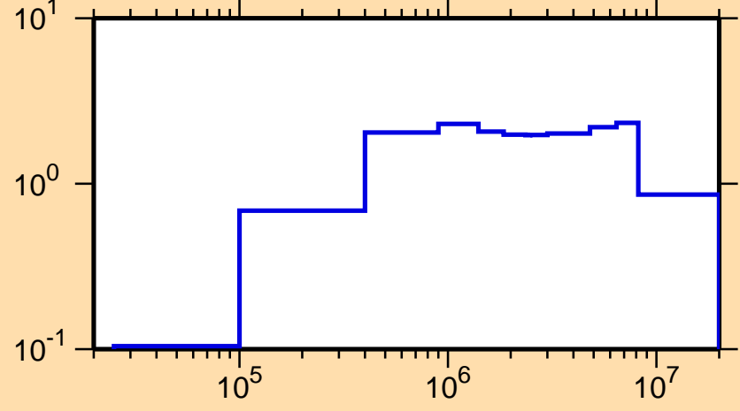
\sigma vs. E for ^{159}\text{Er}(n,\text{inel.})
