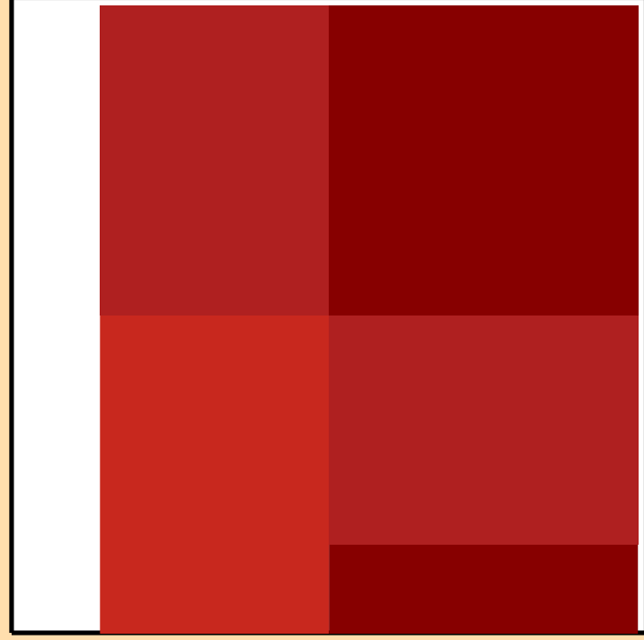
\Delta\sigma/\sigma vs. E for ^{160}\text{Er}(n,2n)
