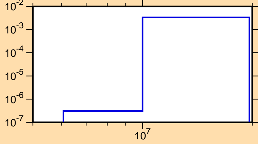
\sigma vs. E for ^{160}\text{Er}(n,np)
