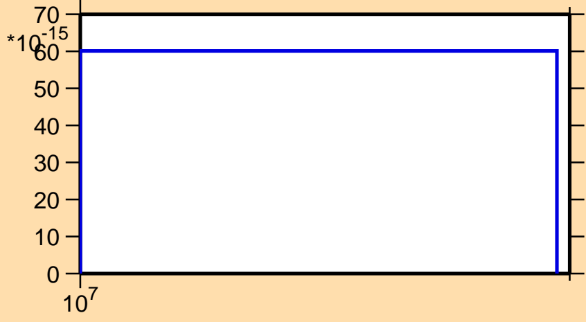
\sigma vs. E for ^{161}\text{Er}(n,\text{pt})
