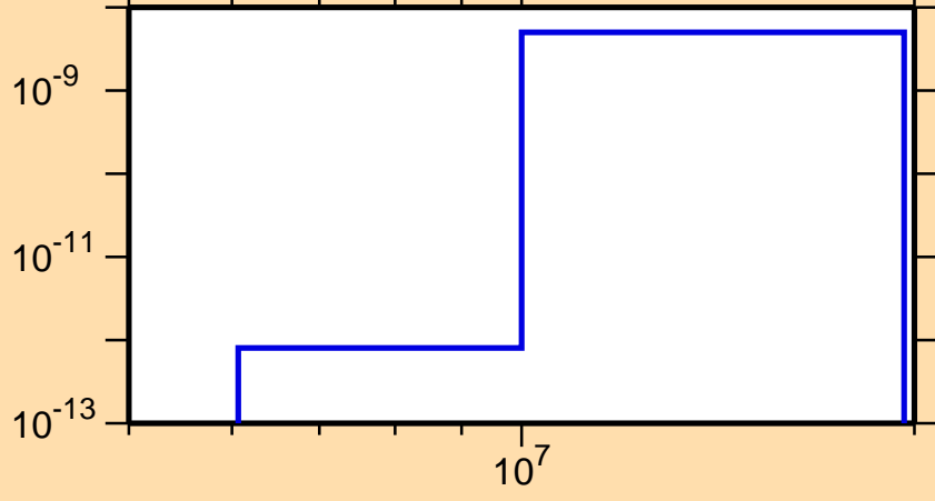
\sigma vs. E for ^{161}\text{Er}(n,p\alpha)
