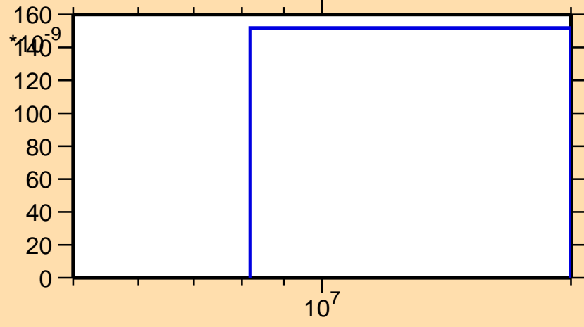
\sigma vs. E for ^{161}\text{Er}(n,2np)
