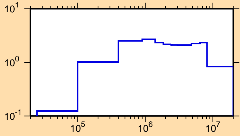
\sigma vs. E for ^{161}\text{Er}(n,\text{inel.})
