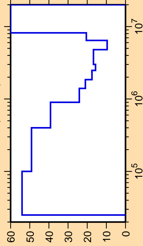
\Delta\sigma/\sigma vs. E for ^{161}\text{Er}(n,\text{inel.})
