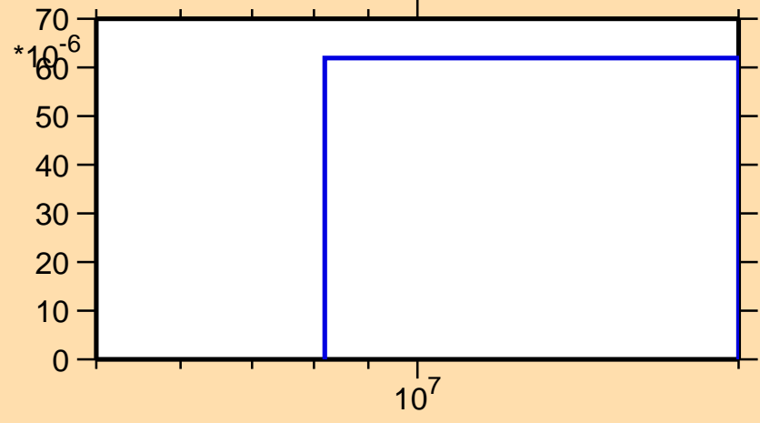
\sigma vs. E for ^{161}\text{Er}(n,t)
