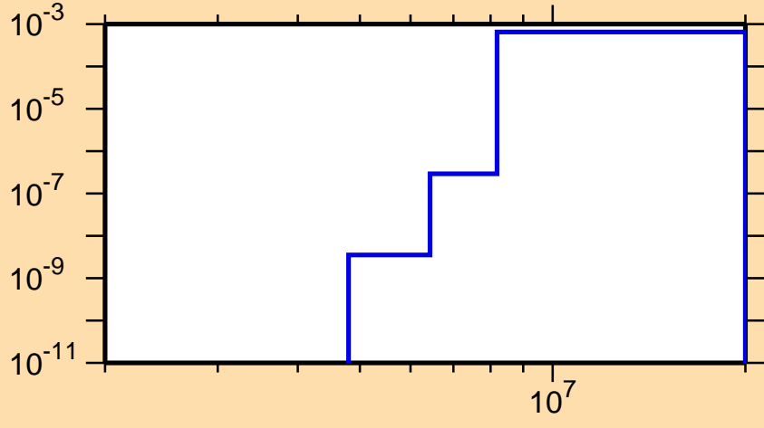
\sigma vs. E for ^{161}\text{Er}(n,n\alpha)
