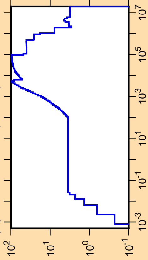
\Delta\mu/\mu vs. E for ^{162}\text{Er}(\text{mt251})
