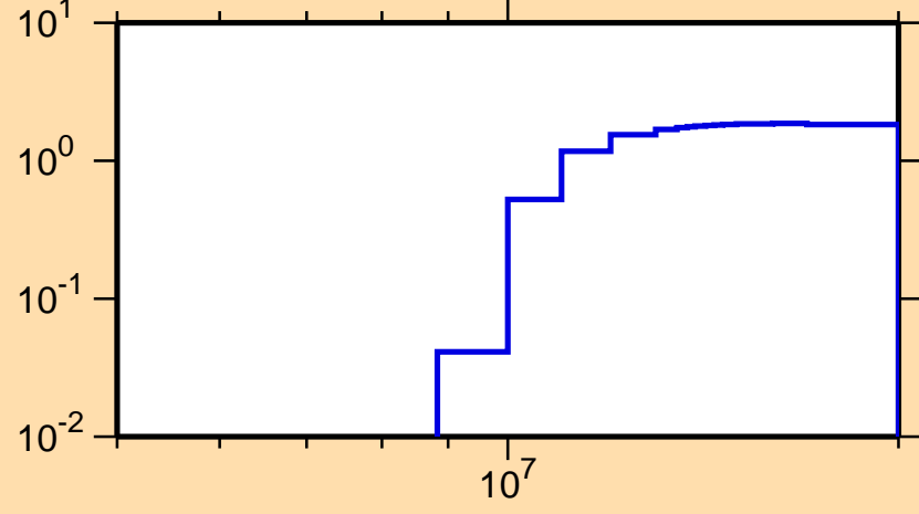
\sigma vs. E for ^{162}\text{Er}(n,2n)
