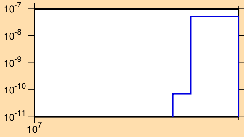
\sigma vs. E for ^{164}\text{Er}(n,\text{nd})
