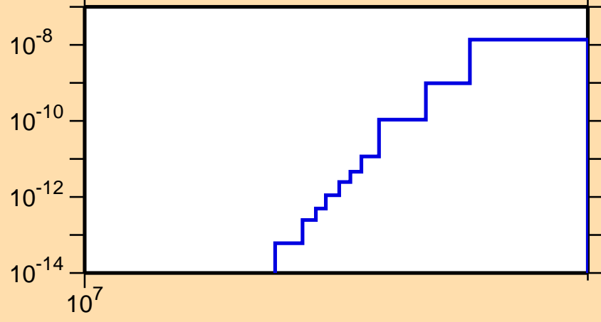
\sigma vs. E for ^{164}\text{Er}(n,\text{He3})
