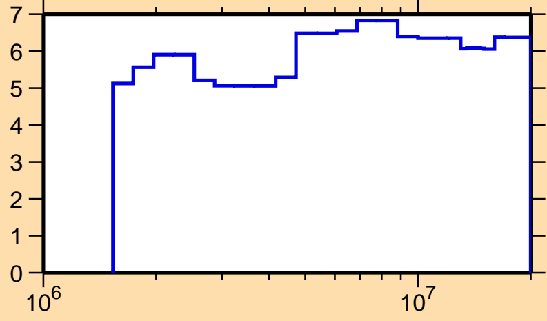
\Delta\sigma/\sigma vs. E for ^{164}\text{Er}(n,n\text{onel.})
