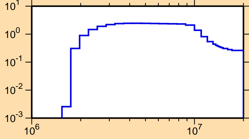
\sigma vs. E for ^{164}\text{Er}(n,n\text{cont.})
