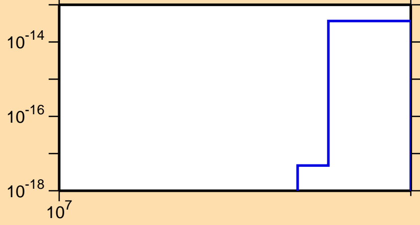
\sigma vs. E for ^{165}\text{Er} (mt 34)
