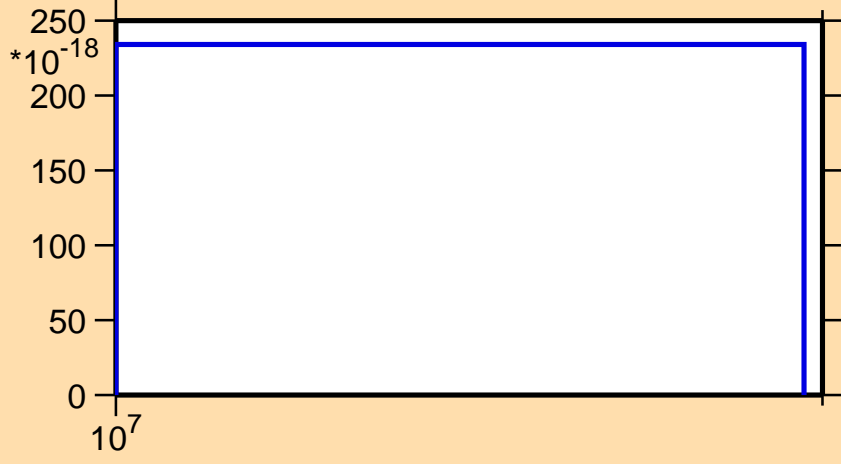
\sigma vs. E for ^{165}\text{Er} (mt 34)
