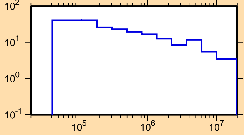
\Delta\sigma/\sigma vs. E for ^{165}\text{Er}(n,\text{tot.})
