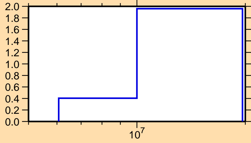
\sigma vs. E for ^{165}\text{Er}(n,2n)
