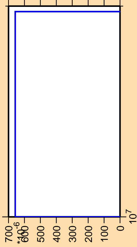
\Delta\sigma/\sigma vs. E for ^{165}\text{Er} (mt 34)
