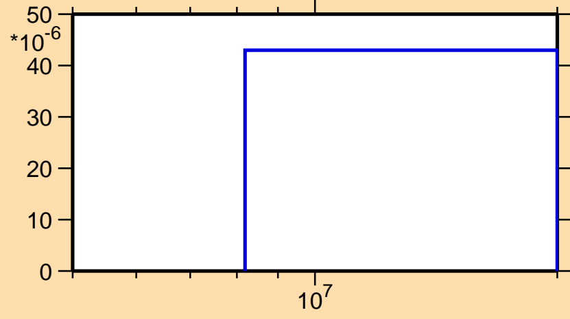
\sigma vs. E for ^{165}\text{Er}(n,t)
