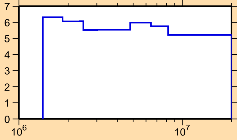
\Delta\sigma/\sigma vs. E for ^{166}\text{Er}(n,n\text{onel.})
