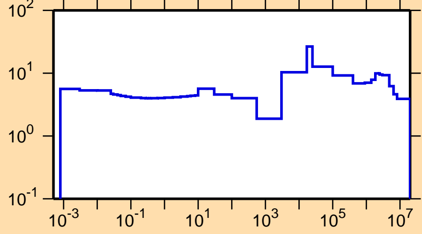
\Delta\sigma/\sigma vs. E for ^{166}\text{Er}(n,\text{tot.})
