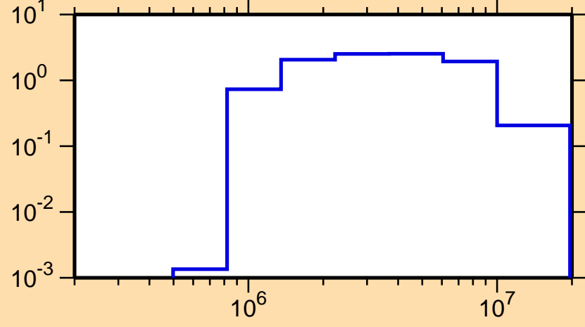
\sigma vs. E for ^{167}\text{Er}(n,n\text{cont.})
