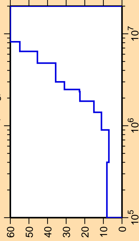
\Delta\sigma/\sigma vs. E for ^{167}\text{Er}(n,n_3)
