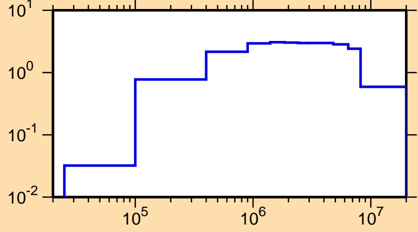
\sigma vs. E for ^{167}\text{Er}(n,\text{inel.})
