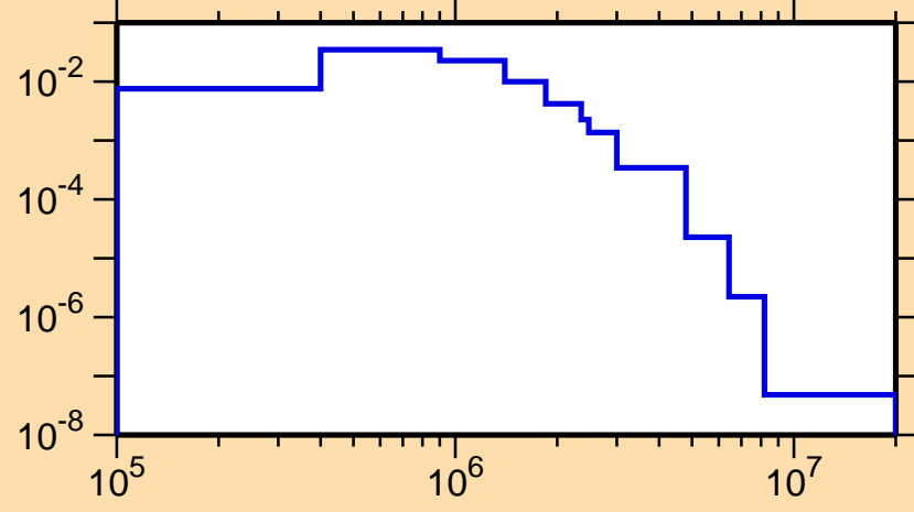
\sigma vs. E for ^{167}\text{Er}(n,n_3)
