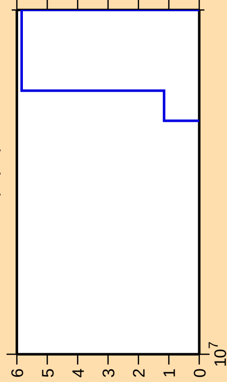
\Delta\sigma/\sigma vs. E for ^{167}\text{Er}(n,p\alpha)
