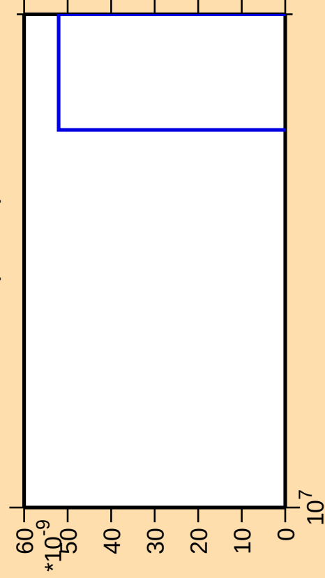
\Delta\sigma/\sigma vs. E for ^{167}\text{Er} (mt 11)
