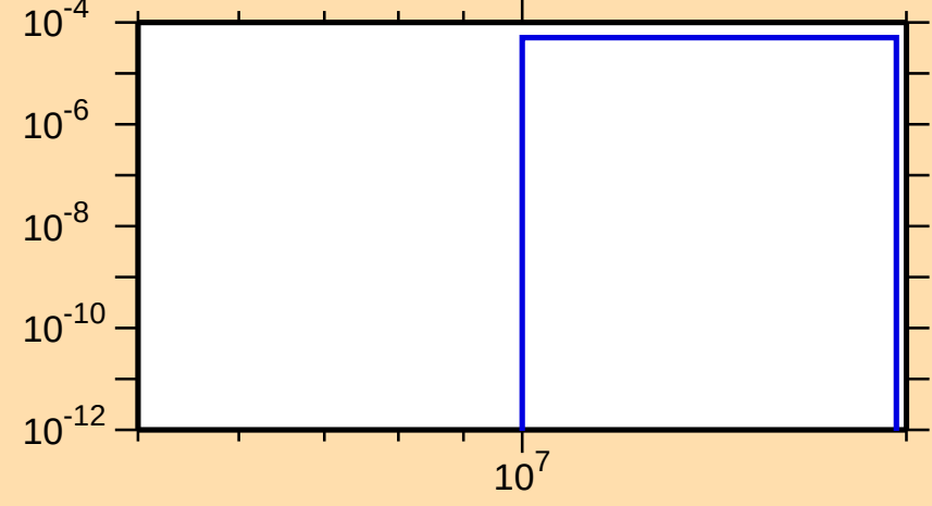
\sigma vs. E for ^{167}\text{Er}(n,t)
