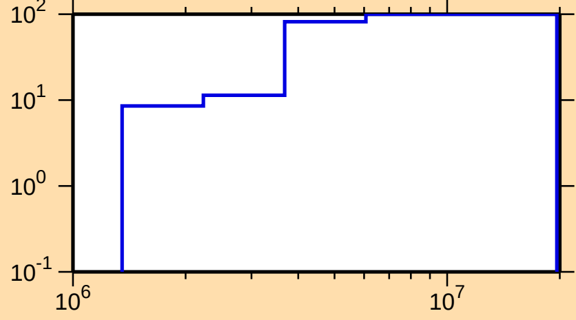
\Delta\sigma/\sigma vs. E for ^{167}\text{Er}(n,n_1)
