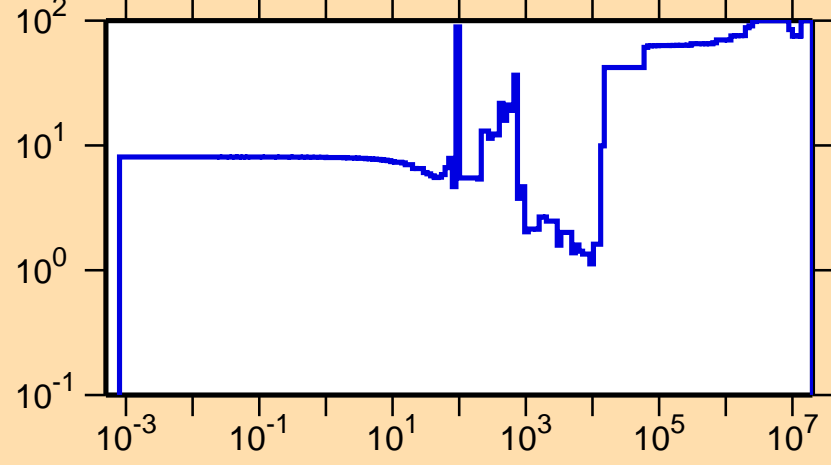
\Delta\sigma/\sigma vs. E for ^{168}\text{Er}(n,\gamma)
