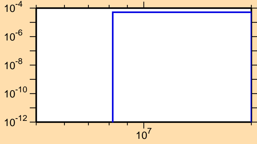
\sigma vs. E for ^{168}\text{Er}(n,np)
