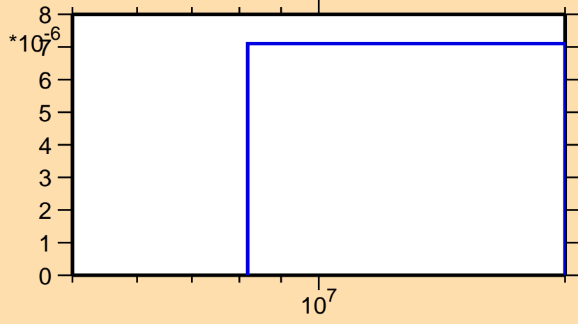
\sigma vs. E for ^{168}\text{Er}(n,t)
