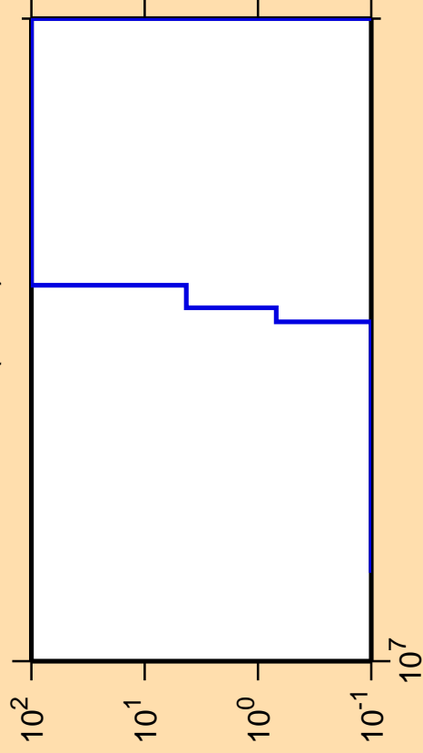
\Delta\sigma/\sigma vs. E for ^{169}\text{Er}(n,nd)
