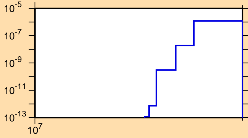
\sigma vs. E for ^{169}\text{Er}(n,nd)
