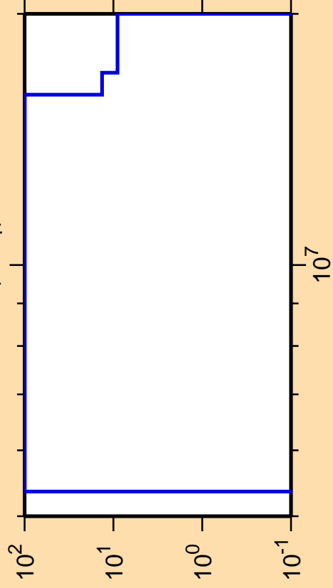
\Delta\sigma/\sigma vs. E for ^{169}\text{Er}(n,n_1)
