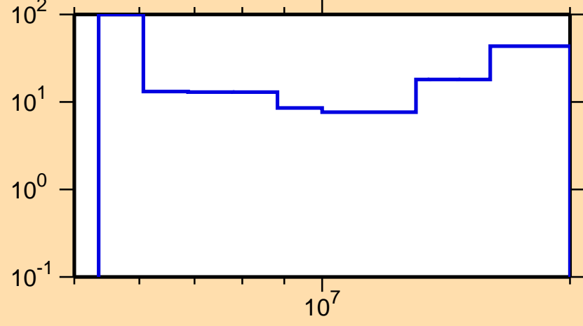
\Delta\sigma/\sigma vs. E for ^{169}\text{Er}(n,2n)
