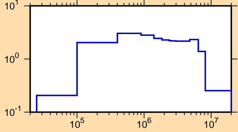
\sigma vs. E for ^{169}\text{Er}(n,\text{inel.})
