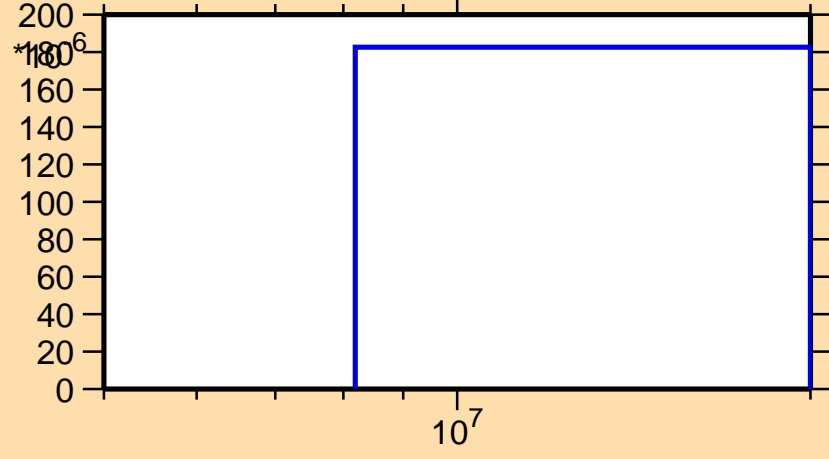
\sigma vs. E for ^{169}\text{Er}(n,d)
