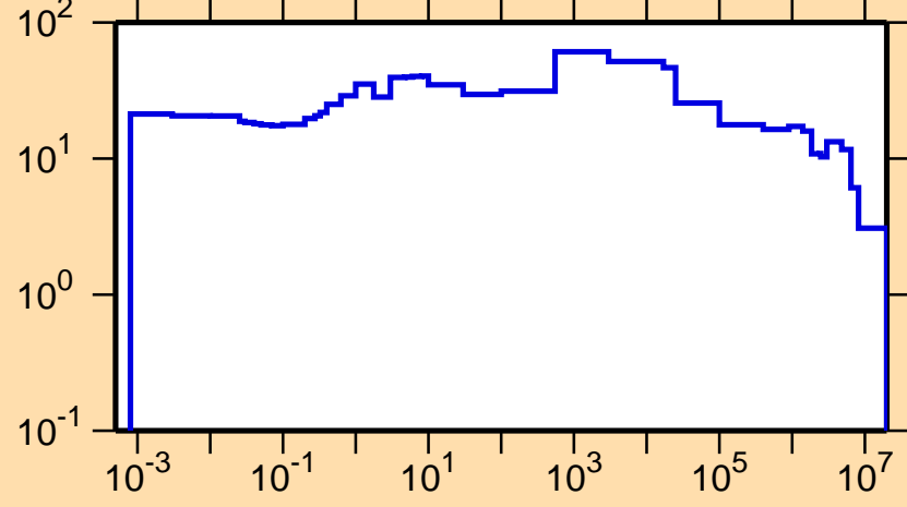
\Delta\sigma/\sigma vs. E for ^{169}\text{Er}(n,\text{tot.})
