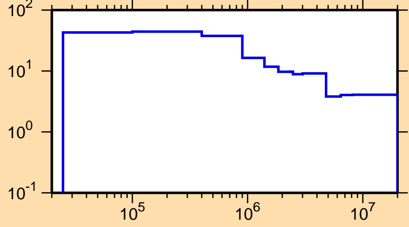
\Delta\sigma/\sigma vs. E for ^{169}\text{Er}(n,\text{nonel.})
