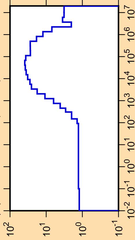
\Delta\mu/\mu vs. E for ^{170}\text{Er}(\text{mt251})
