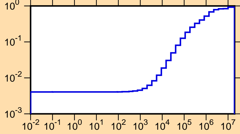
\mu vs. E for ^{170}\text{Er}(\text{mt251})
