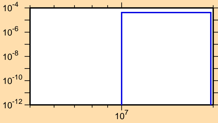
\sigma vs. E for ^{170}\text{Er}(n,np)
