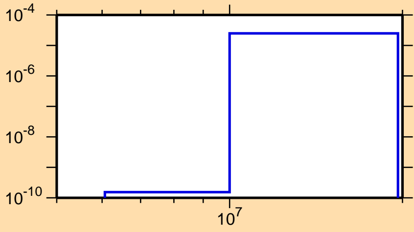
\sigma vs. E for ^{170}\text{Er}(n,\alpha)
