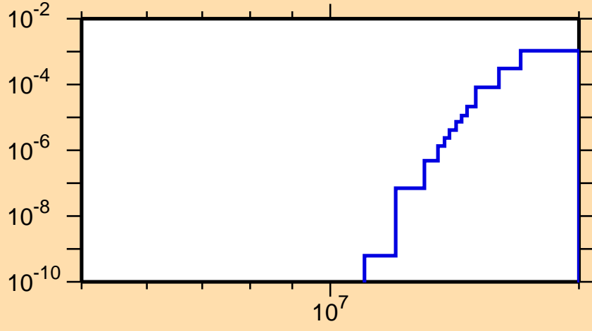
\sigma vs. E for ^{171}\text{Er}(n,np)
