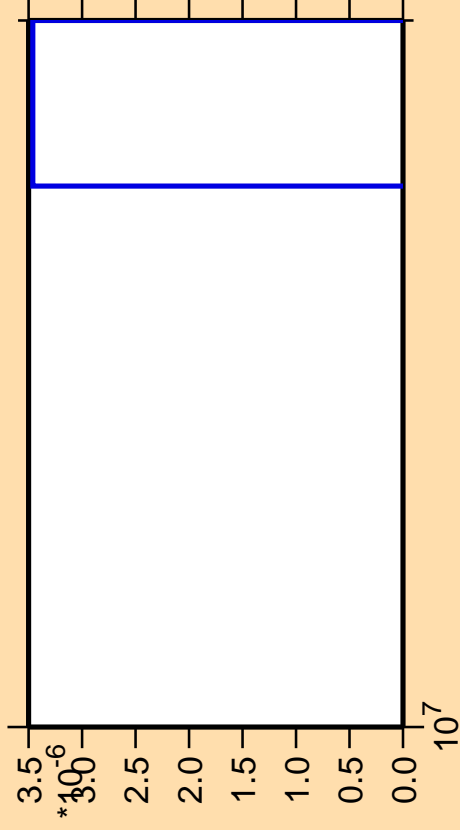
\Delta\sigma/\sigma vs. E for ^{171}\text{Er}(\text{mt } 11)
