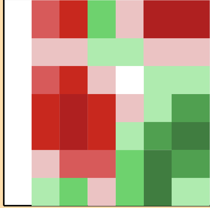
\Delta\sigma/\sigma vs. E for ^{171}\text{Er}(n,n\text{cont.})
