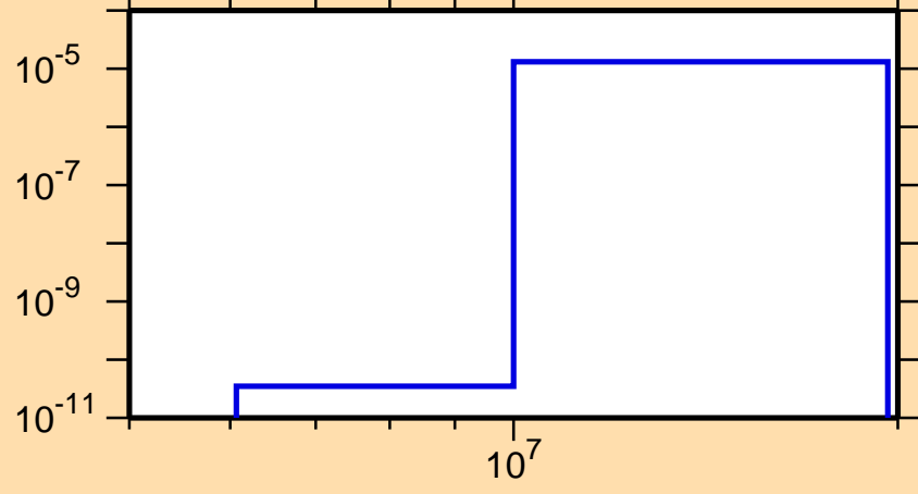
\sigma vs. E for ^{171}\text{Er}(n,\alpha)
