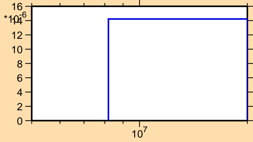
\sigma vs. E for ^{171}\text{Er}(n,t)
