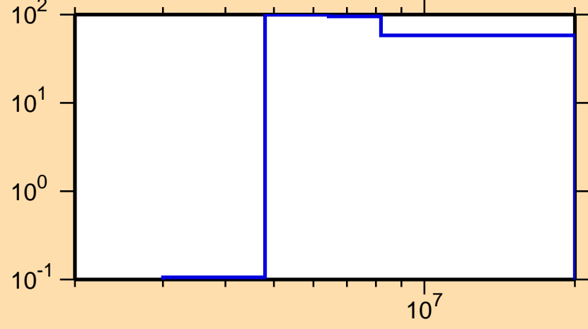
\Delta\sigma/\sigma vs. E for ^{171}\text{Er}(n,p)
