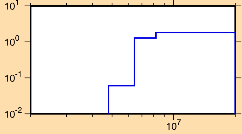
\sigma vs. E for ^{171}\text{Er}(n,2n)
