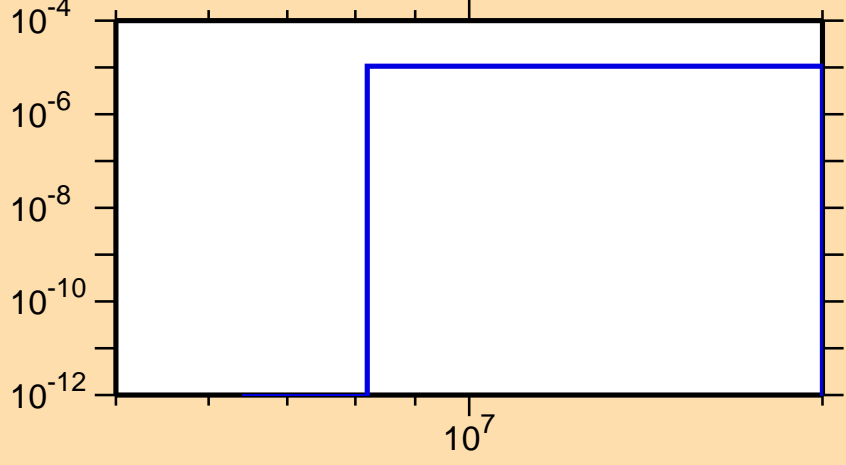
\sigma vs. E for ^{171}\text{Er}(n,\alpha)
