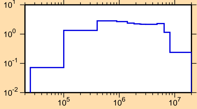
\sigma vs. E for ^{171}\text{Er}(n,\text{inel.})
