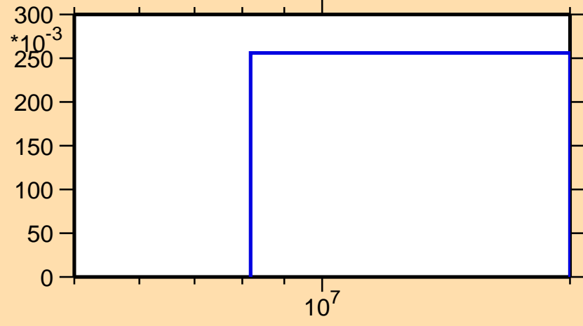
\sigma vs. E for ^{171}\text{Er}(n,3n)
