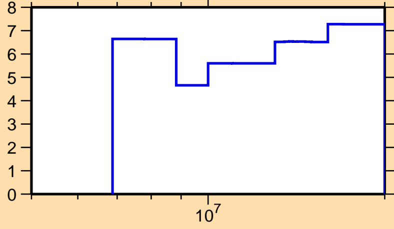
\Delta\sigma/\sigma vs. E for ^{172}\text{Er}(n,\text{tot.})
