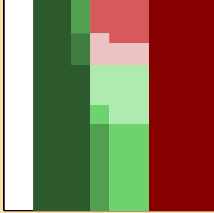
\Delta\sigma/\sigma vs. E for ^{172}\text{Er}(n,p)
