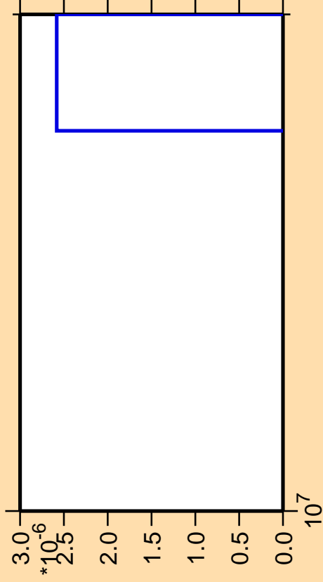
\Delta\sigma/\sigma vs. E for ^{172}\text{Er} (mt 11)
