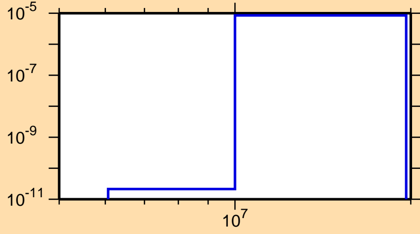
\sigma vs. E for ^{172}\text{Er}(n,\alpha)
