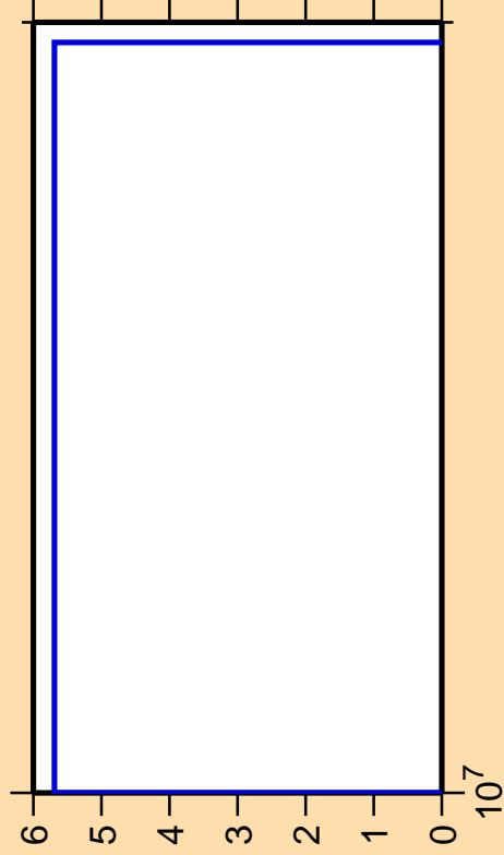
\Delta\sigma/\sigma vs. E for ^{172}\text{Er}(n,2np)
