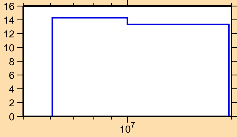
\Delta\sigma/\sigma vs. E for ^{172}\text{Er}(n,el.)
