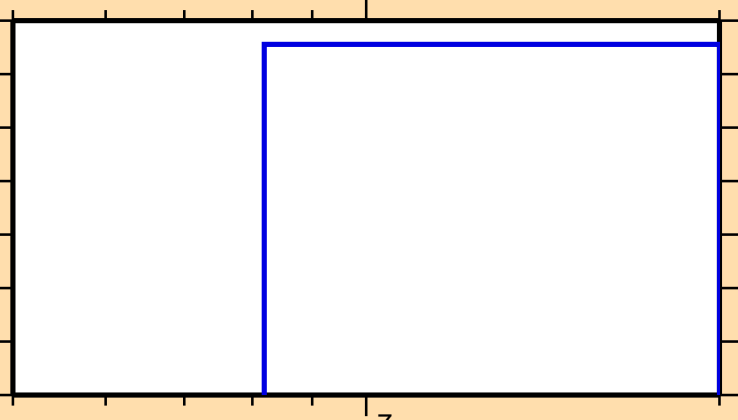
\sigma vs. E for ^{172}\text{Er}(n,np)
