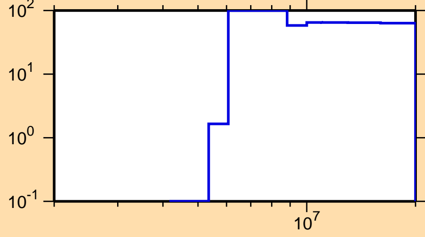
\Delta\sigma/\sigma vs. E for ^{173}\text{Er}(n,p)
