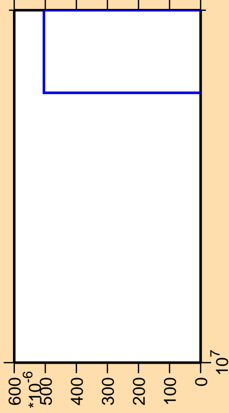
\Delta\sigma/\sigma vs. E for ^{173}\text{Er} (mt 11)
