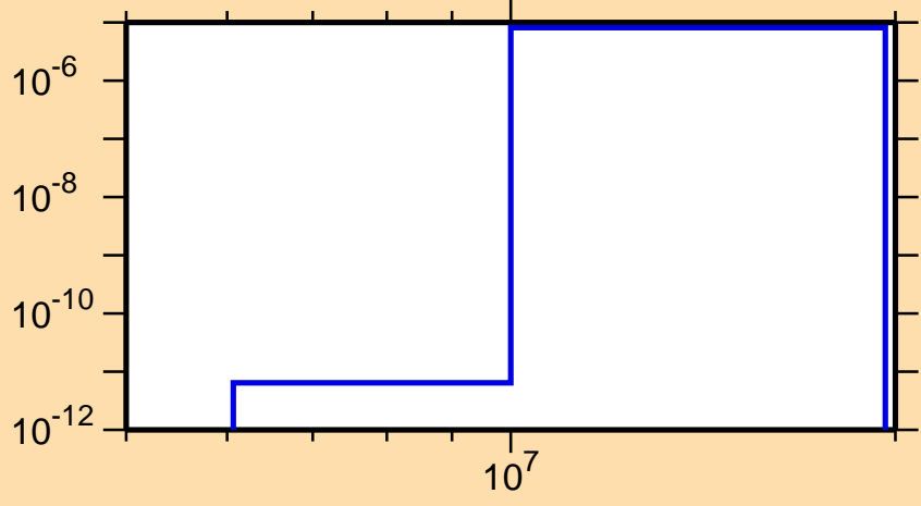
\sigma vs. E for ^{173}\text{Er}(n,\alpha)
