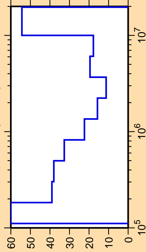
\Delta\sigma/\sigma vs. E for ^{173}\text{Er}(n,\text{inel.})
