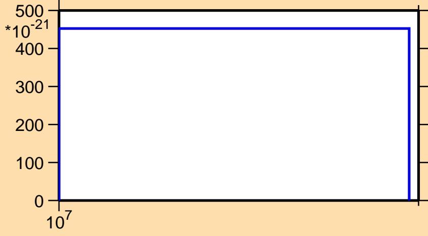
\sigma vs. E for ^{173}\text{Er} (mt 11)
