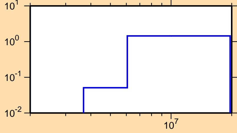
\sigma vs. E for ^{173}\text{Er}(n,2n)
