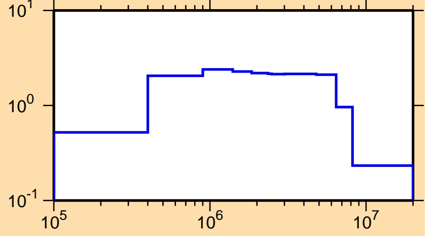
\sigma vs. E for ^{173}\text{Er}(n,\text{inel.})
