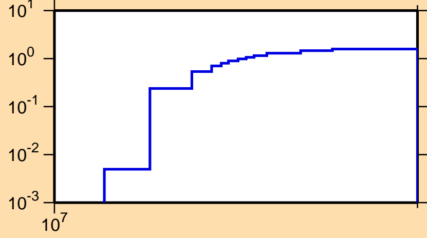
\sigma vs. E for ^{174}\text{Er}(n,3n)
