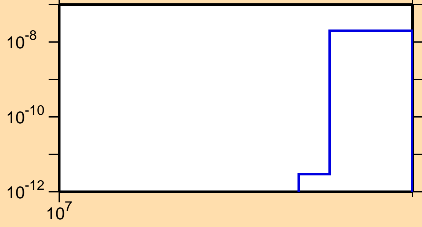
\sigma vs. E for ^{174}\text{Er}(n,\text{nd})
