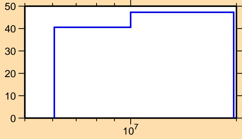
\Delta\sigma/\sigma vs. E for ^{174}\text{Er}(n,ncont.)
