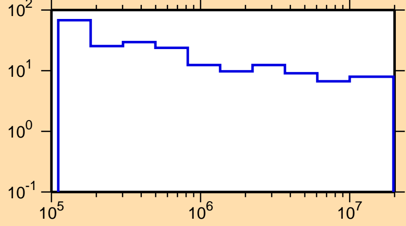
\Delta\sigma/\sigma vs. E for ^{174}\text{Er}(n,\text{nonel.})
