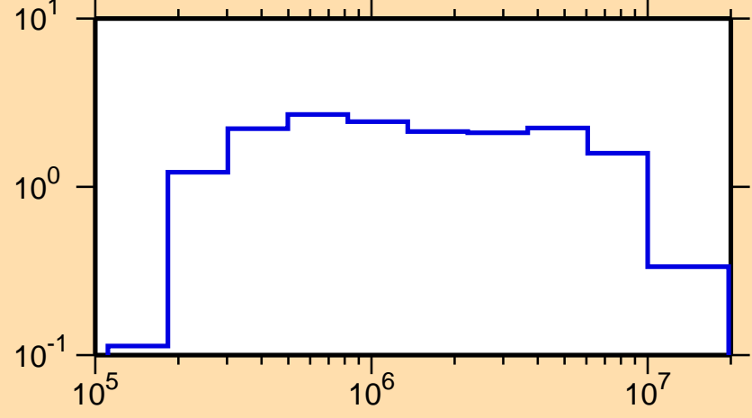
\sigma vs. E for ^{174}\text{Er}(n,\text{inel.})
