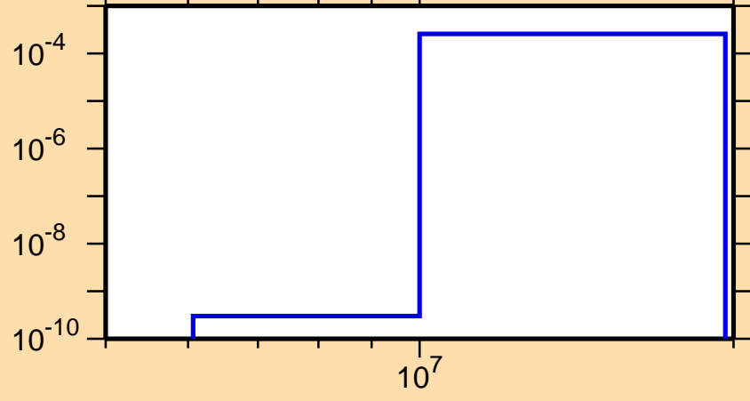
\sigma vs. E for ^{174}\text{Er}(n,p)
