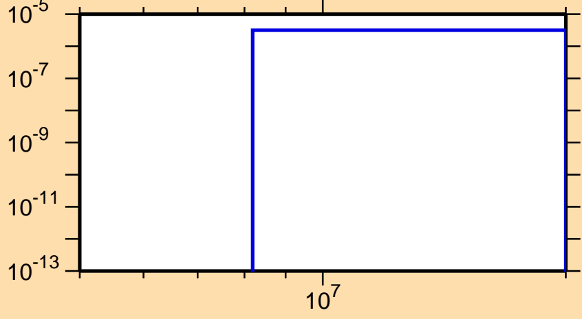
\sigma vs. E for ^{174}\text{Er}(n,\alpha)
