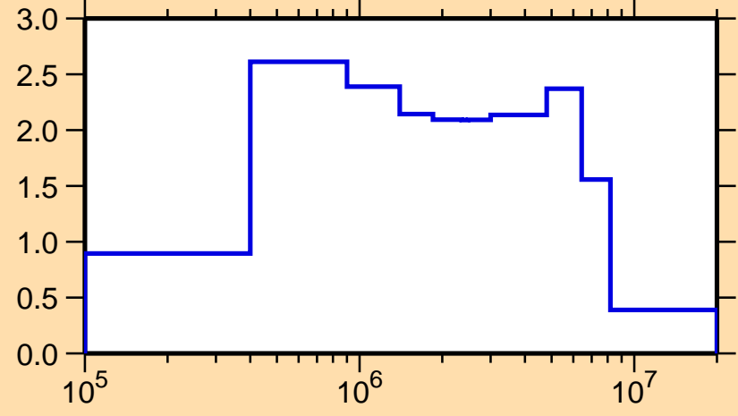
\sigma vs. E for ^{174}\text{Er}(n,\text{inel.})
