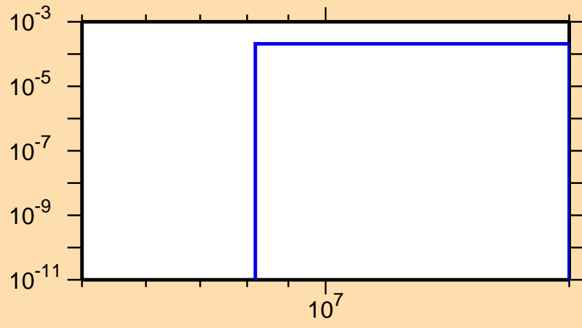
\sigma vs. E for ^{174}\text{Er}(n,p)
