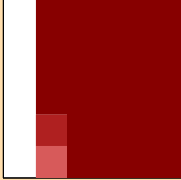
\Delta\sigma/\sigma vs. E for ^{174}\text{Er}(n,p)
