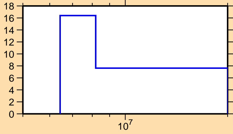
\Delta\sigma/\sigma vs. E for ^{174}\text{Er}(n,el.)
