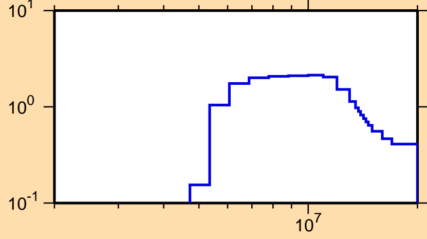
\sigma vs. E for ^{175}\text{Er}(n,2n)
