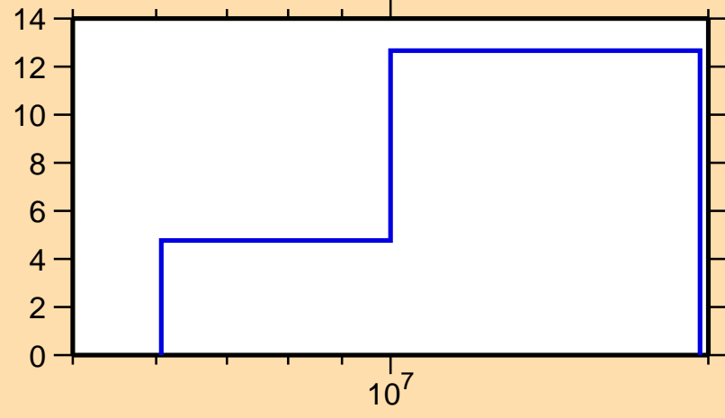
\Delta\sigma/\sigma vs. E for ^{175}\text{Er}(n,el.)
