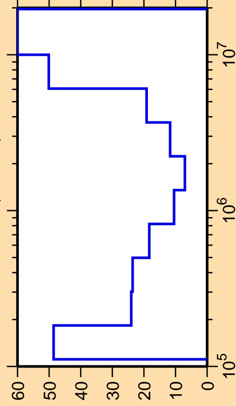
\Delta\sigma/\sigma vs. E for ^{175}\text{Er}(n,\text{inel.})
