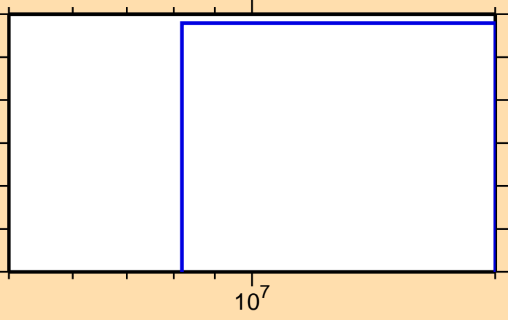
\sigma vs. E for ^{175}\text{Er}(n,2n\alpha)
