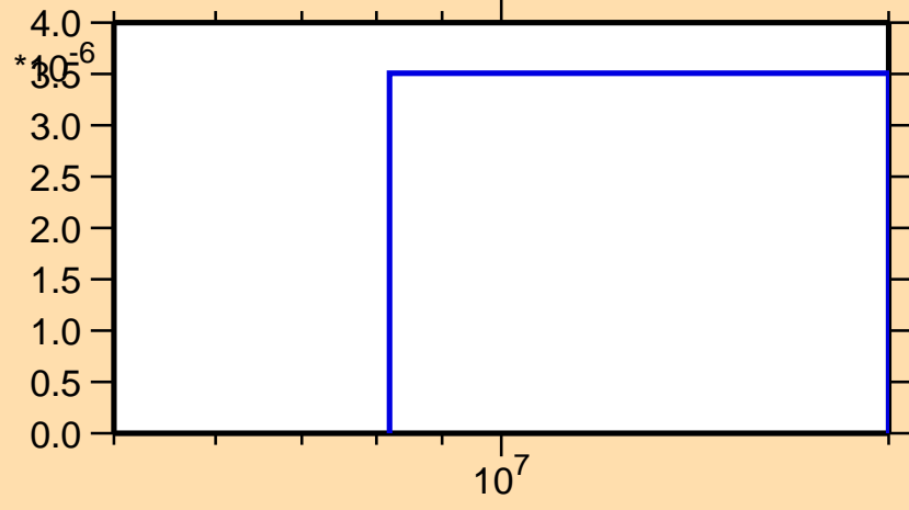
\sigma vs. E for ^{175}\text{Er}(n,\alpha)
