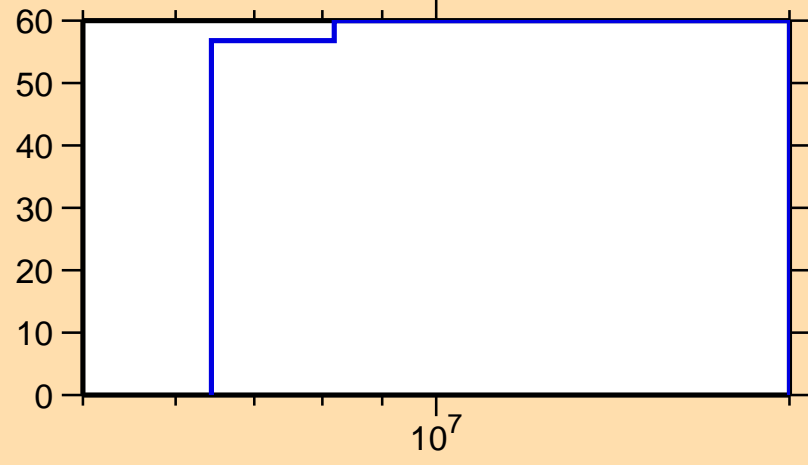
\Delta\sigma/\sigma vs. E for ^{175}\text{Er}(n,ncont.)
