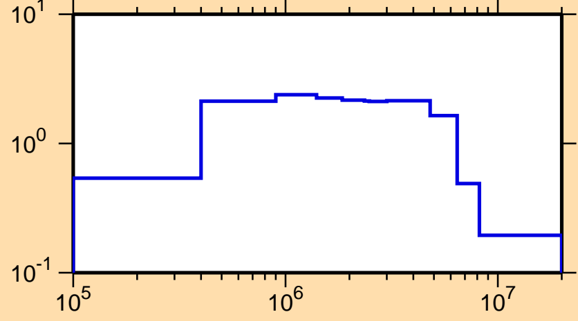
\sigma vs. E for ^{175}\text{Er}(n,\text{inel.})
