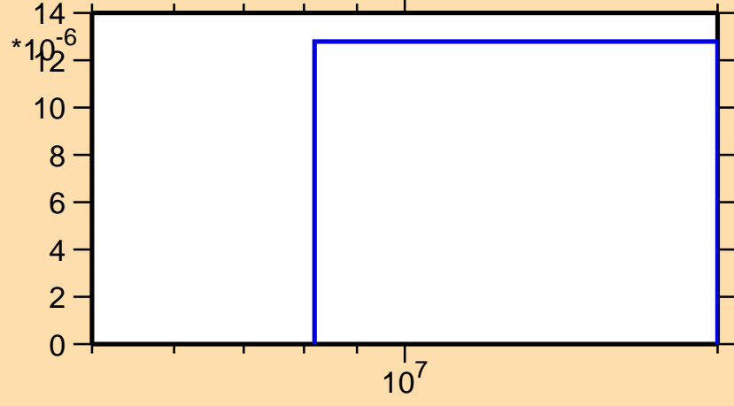
\sigma vs. E for ^{175}\text{Er}(n,d)
