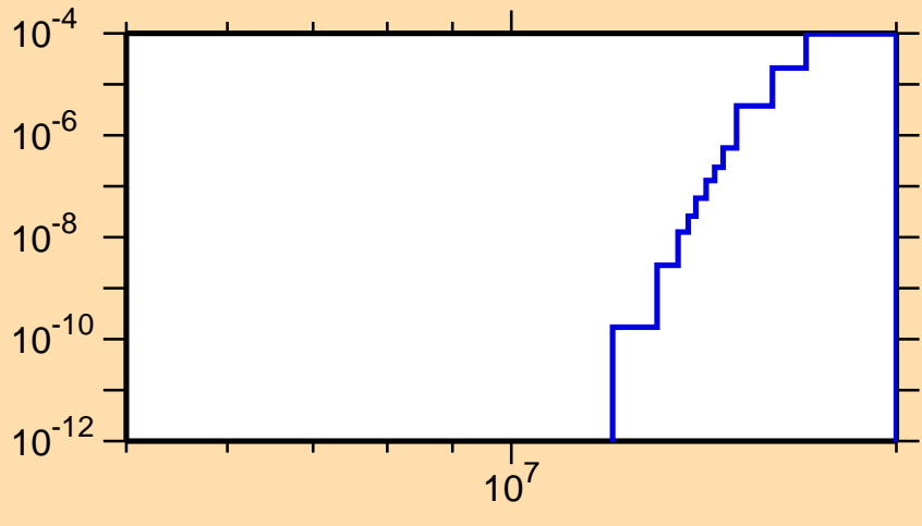
\sigma vs. E for ^{176}\text{Er}(n,t)
