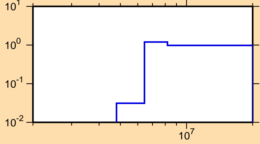
\sigma vs. E for ^{176}\text{Er}(n,2n)
