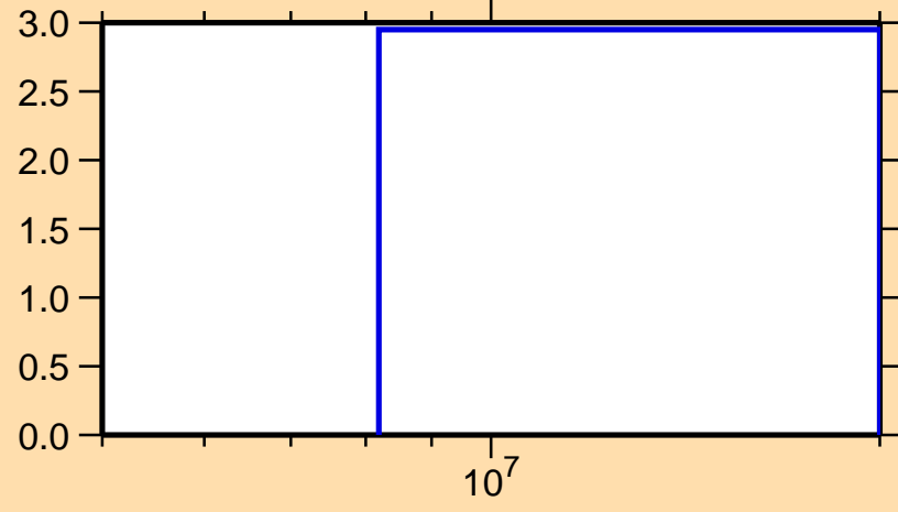
\Delta\sigma/\sigma vs. E for ^{176}\text{Er}(n,el.)
