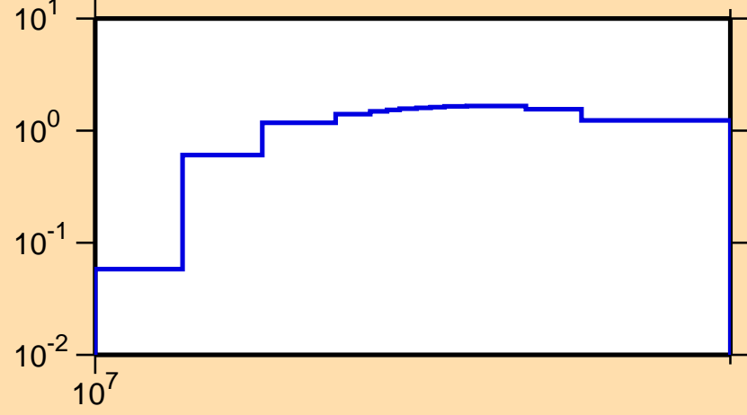
\sigma vs. E for ^{177}\text{Er}(n,3n)
