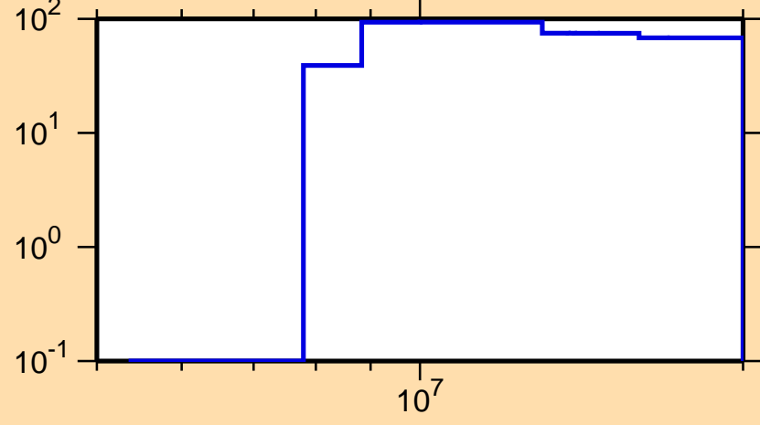
\Delta\sigma/\sigma vs. E for ^{177}\text{Er}(n,p)
