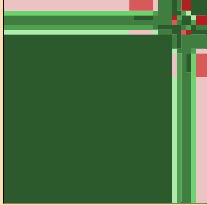
\mu vs. E for ^{177}\text{Er}(\text{mt251})
