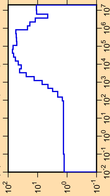
\Delta\mu/\mu vs. E for ^{177}\text{Er}(\text{mt251})
