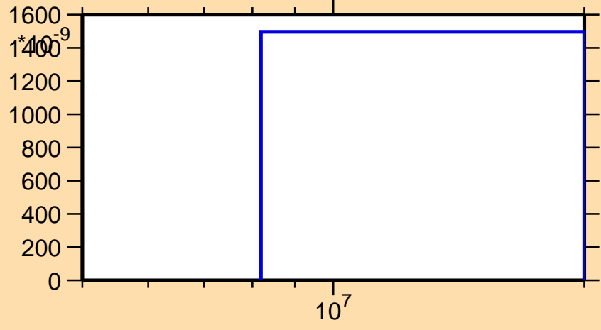
\sigma vs. E for ^{177}\text{Er}(n,\alpha)
