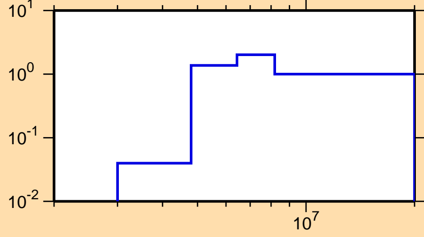
\sigma vs. E for ^{177}\text{Er}(n,2n)
