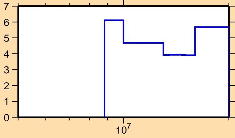
\Delta\sigma/\sigma vs. E for ^{239}\text{Es}(n,\text{el.})
