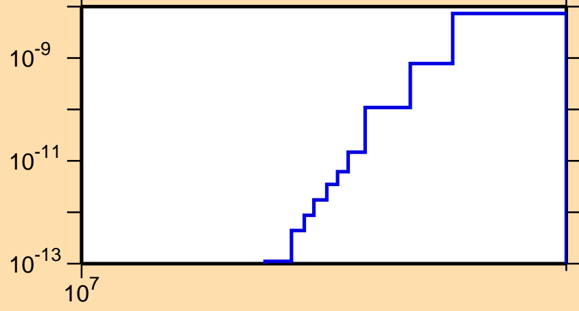
\sigma vs. E for ^{239}\text{Es}(n,nd)
