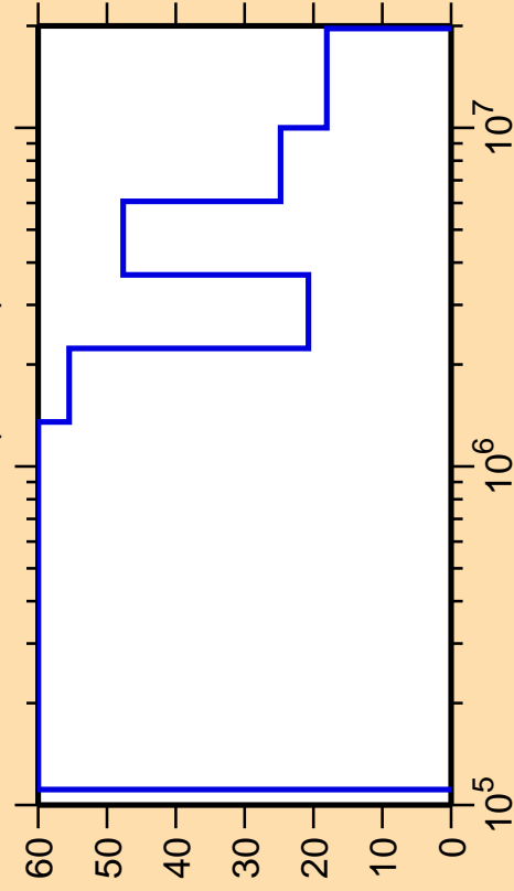
\Delta\sigma/\sigma vs. E for ^{239}\text{Es}(n,\text{inel.})
