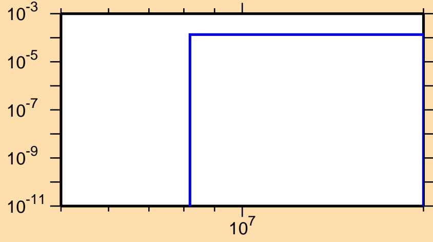
\sigma vs. E for ^{239}\text{Es}(n,t)
