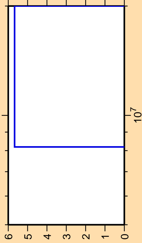
\Delta\sigma/\sigma vs. E for ^{239}\text{Es}(n,nt)
