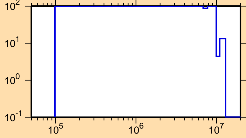
\Delta\sigma/\sigma vs. E for ^{240}\text{Es}(n,n_1)
