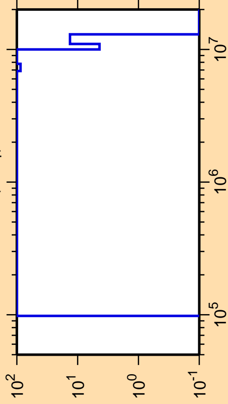
\Delta\sigma/\sigma vs. E for ^{240}\text{Es}(n,n_1)
