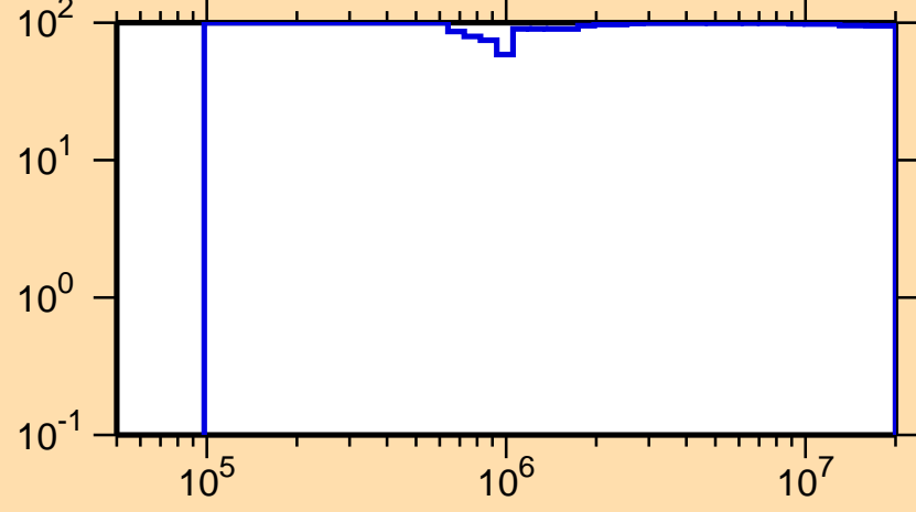
\Delta\sigma/\sigma vs. E for ^{240}\text{Es}(n,n\text{cont.})
