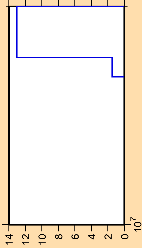
\Delta\sigma/\sigma vs. E for ^{240}\text{Es}(n,\text{pd})
