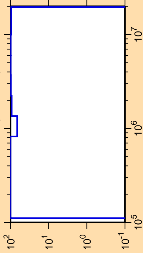
\Delta\sigma/\sigma vs. E for ^{240}\text{Es}(n,\text{ncont.})
