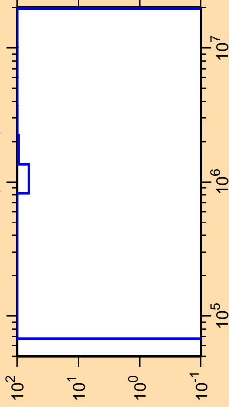
\Delta\sigma/\sigma vs. E for ^{240}\text{Es}(n,\text{inel.})
