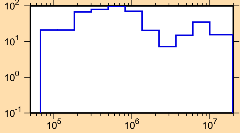
\Delta\sigma/\sigma vs. E for ^{240}\text{Es}(n,\text{el.})
