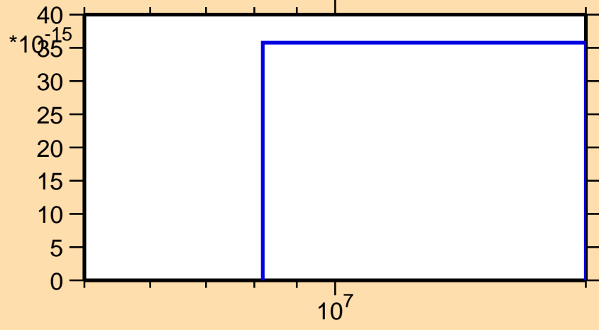
\sigma vs. E for ^{240}\text{Es}(n,\text{pd})
