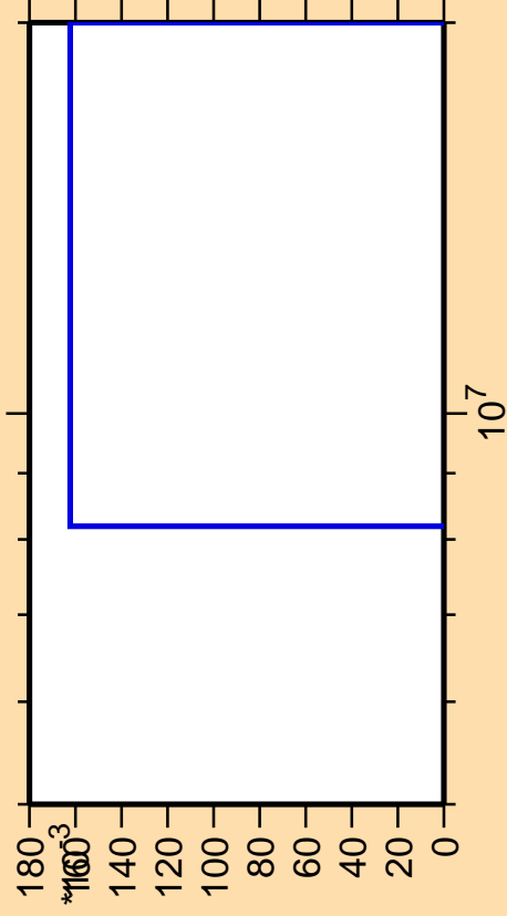
\Delta\sigma/\sigma vs. E for ^{240}\text{Es}(n,\text{pd})
