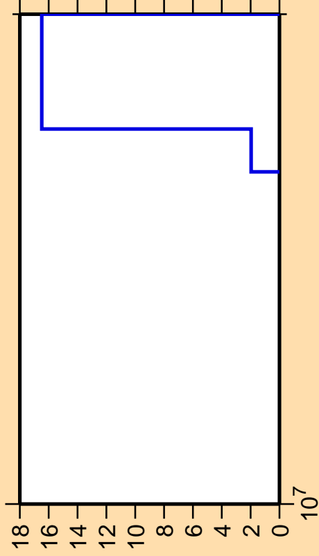
\Delta\sigma/\sigma vs. E for ^{241}\text{Es}(n,\text{pd})
