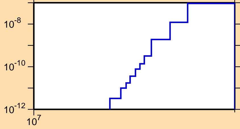
\sigma vs. E for ^{241}\text{Es}(n,nd)
