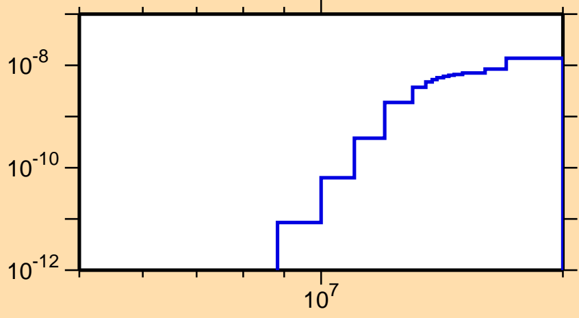
\sigma vs. E for ^{241}\text{Es}(n,2n\alpha)
