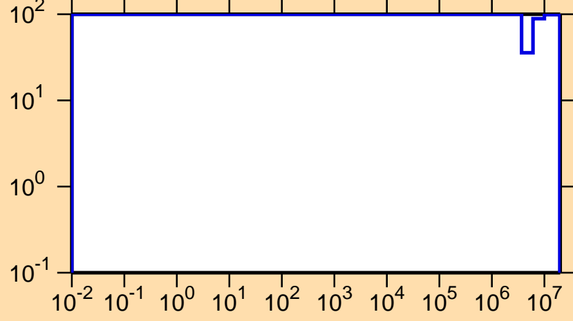
\Delta\sigma/\sigma vs. E for ^{241}\text{Es}(n,p)
