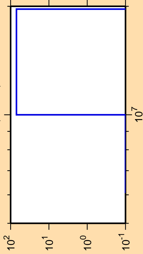
\Delta\sigma/\sigma vs. E for ^{241}\text{Es} (mt 45)
