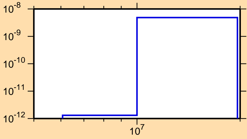
\sigma vs. E for ^{241}\text{Es}(n,2n\alpha)
