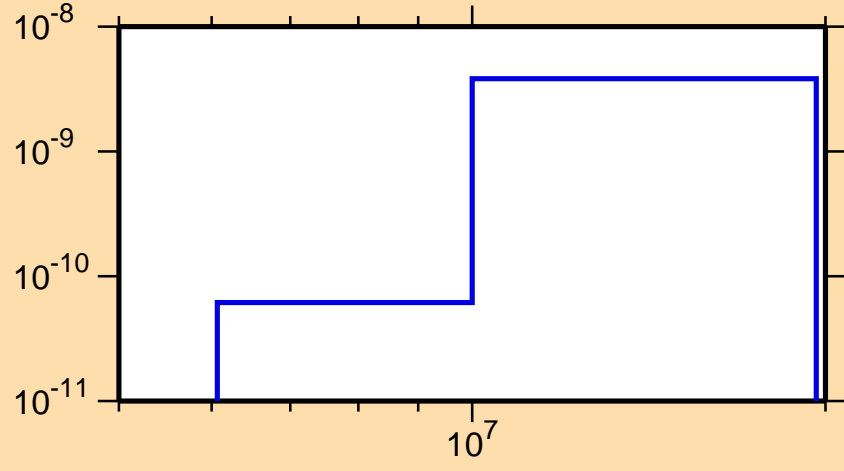
\sigma vs. E for ^{241}\text{Es}(n,p\alpha)
