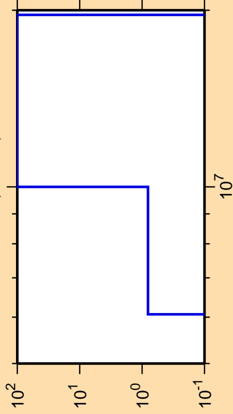
\Delta\sigma/\sigma vs. E for ^{241}\text{Es}(n,2n\alpha)
