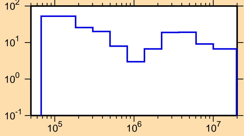
\Delta\sigma/\sigma vs. E for ^{241}\text{Es}(n,\text{tot.})
