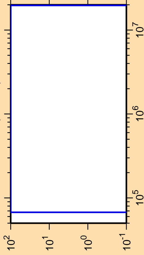
\Delta\sigma/\sigma vs. E for ^{241}\text{Es}(n,\text{inel.})
