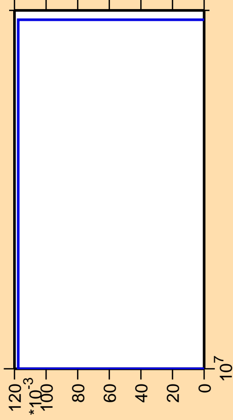
\Delta\sigma/\sigma vs. E for ^{241}\text{Es} (mt 34)
