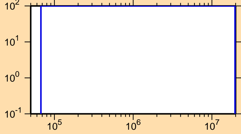
\Delta\sigma/\sigma vs. E for ^{241}\text{Es}(n,\text{inel.})
